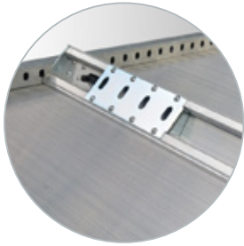
Accessorie: wheelstop with tie-down possibilities
