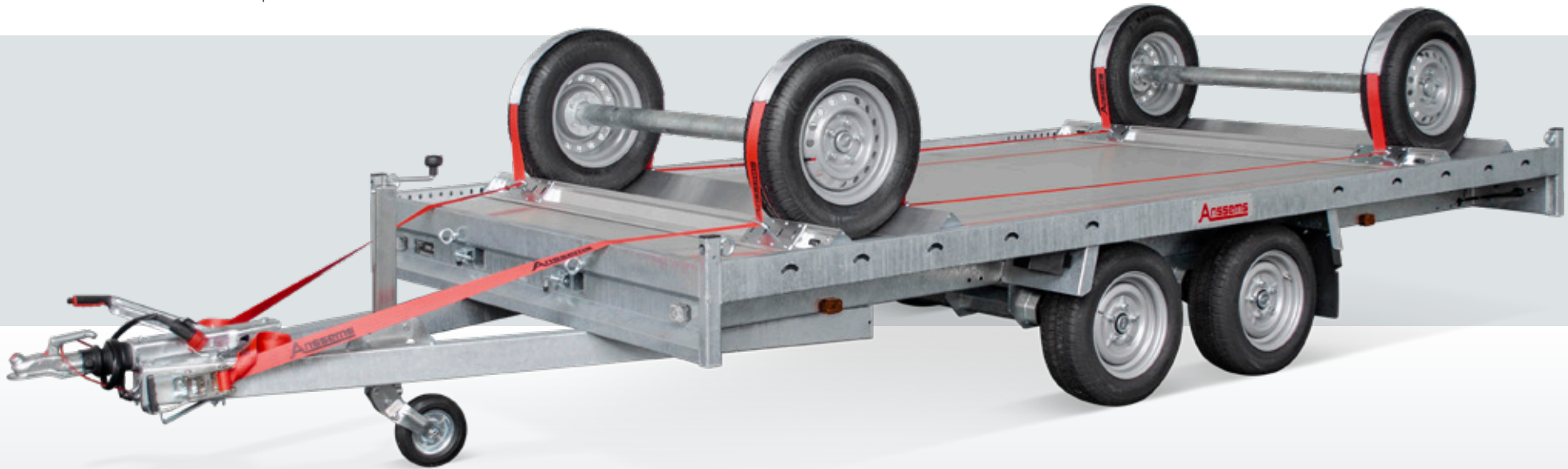
Accessorie: wheelstop with tie-down possibilities
